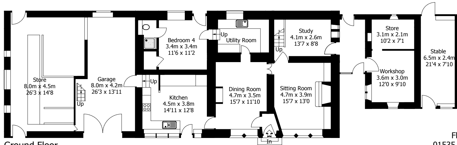
Ground Floor
