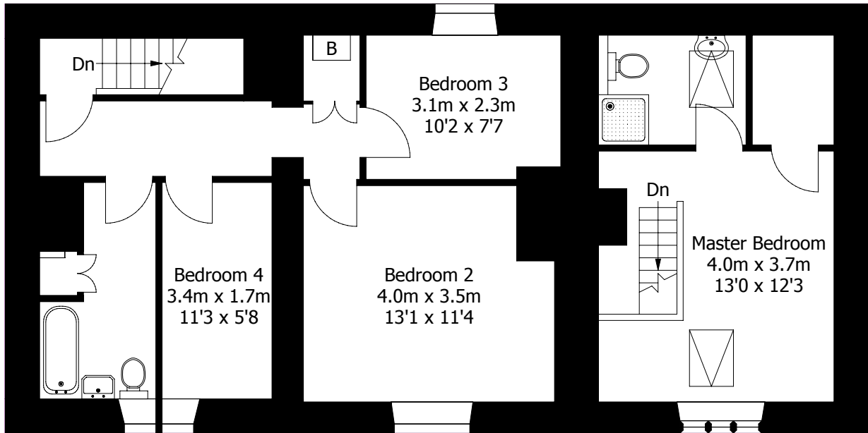
First Floor
